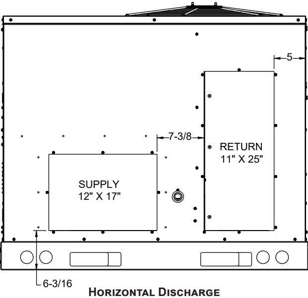
HORIZONTAL DISCHARGE
