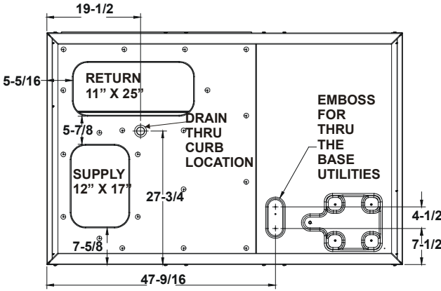
BOTTOM VIEW OF UNIT VERTICAL DISCHARGE
